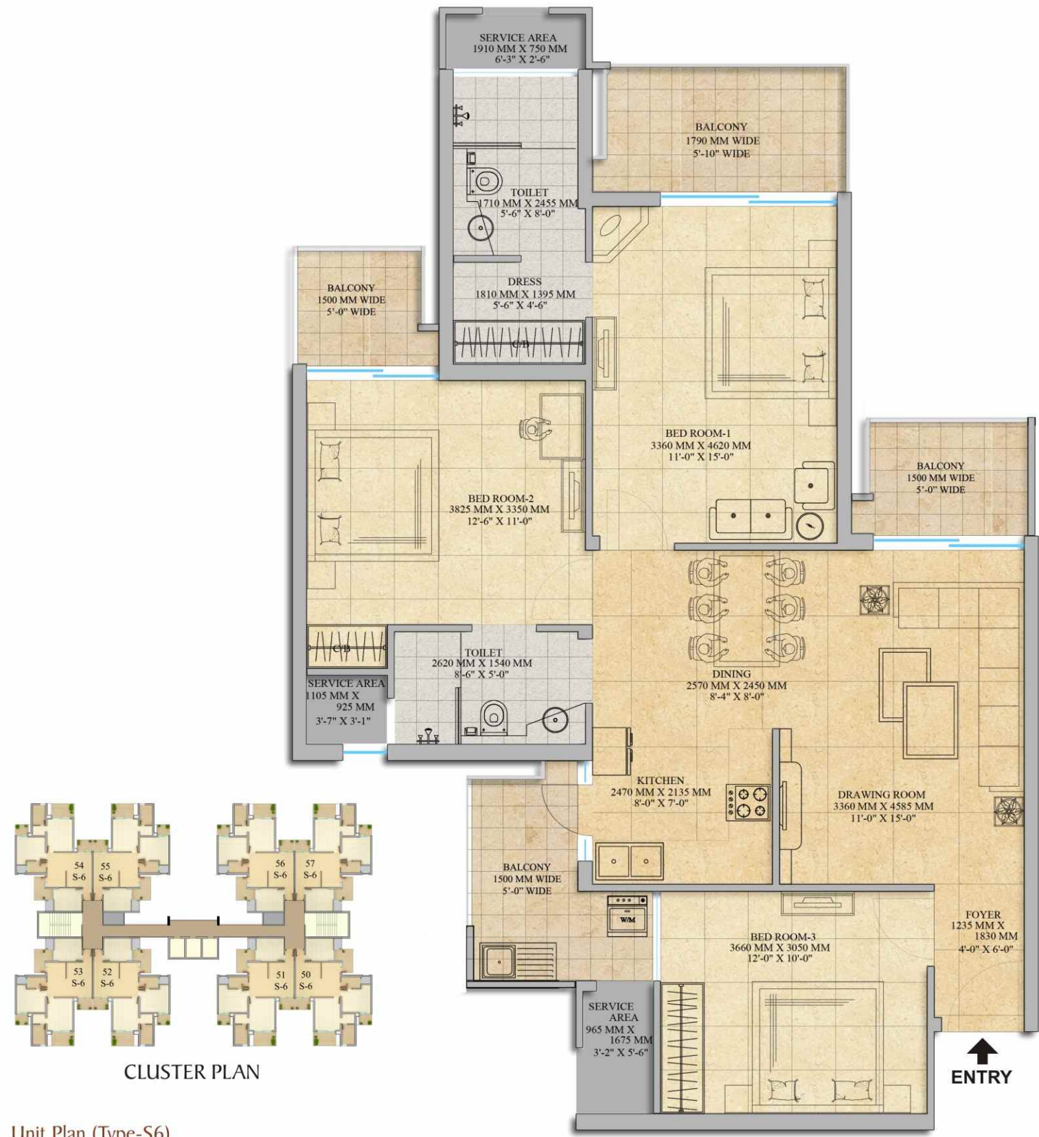
Unit Plan (Type-S6) Magnolia Towers (25+21 Floors) Super Built-up Area = 144.00 Sq. Mt. / 1550.00 Sq. Ft. Coved. Area (R.C.C. Slab Area of flat) = 114.920 Sq. Mt. / 1236.00 Sq. Ft. 3 Bedrooms+Living+Dining+Kitchen+2 Toilets+ 1 Dressing+Entrance Foyer+Balcony+Service Area
